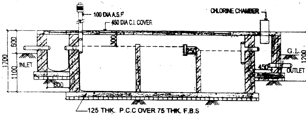
SECTION X-X
